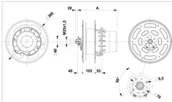
A = 330 mm
